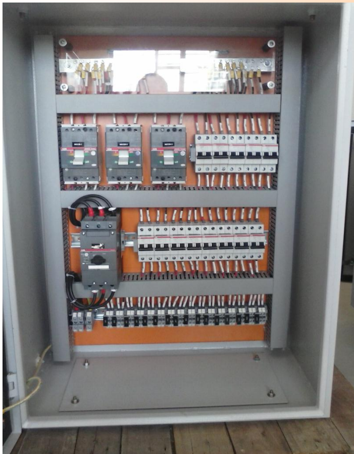
Lighting Distribution Panel
